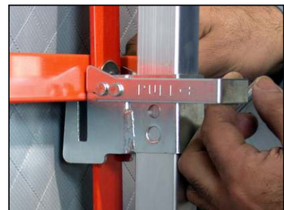
STF18-RUB Roll-up sign bracket
